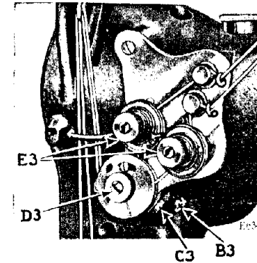
Fig. 19. Adjustment of Thread Controller on Machines of Class 46w
