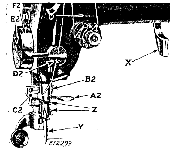
Fig. 25. Adjustments on the Trimmer of Machine 47w64
