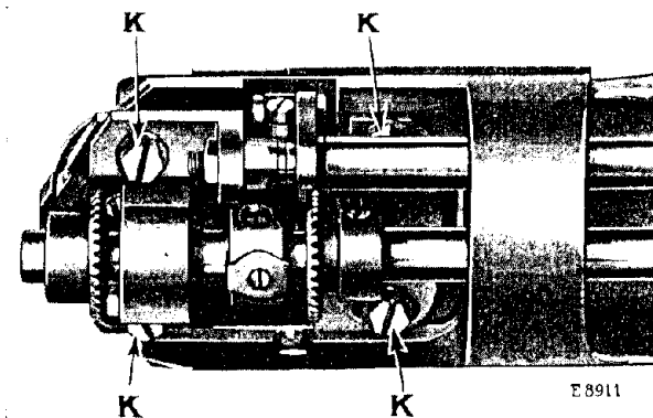
Fig. 21. Adjustment of Hook Saddles
