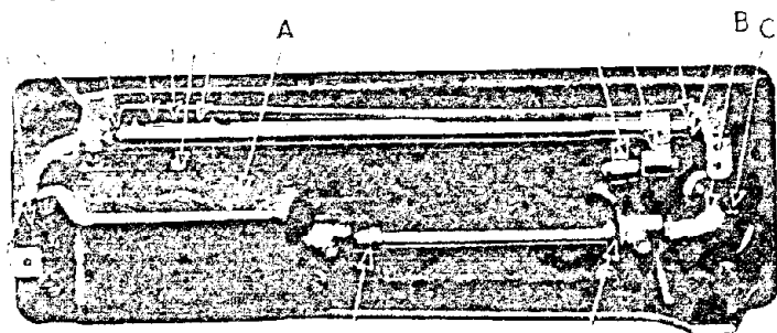
Fig. 5. Base of Machine, Showing Oiling Points. The gear case (B, Fig. 5) should be removed occasionally and filled with the Singer High Speed Lubricant, a grease which is especially prepared for the purpose. The gear case can be easily removed after taking out the screw (C, Fig. 5).
