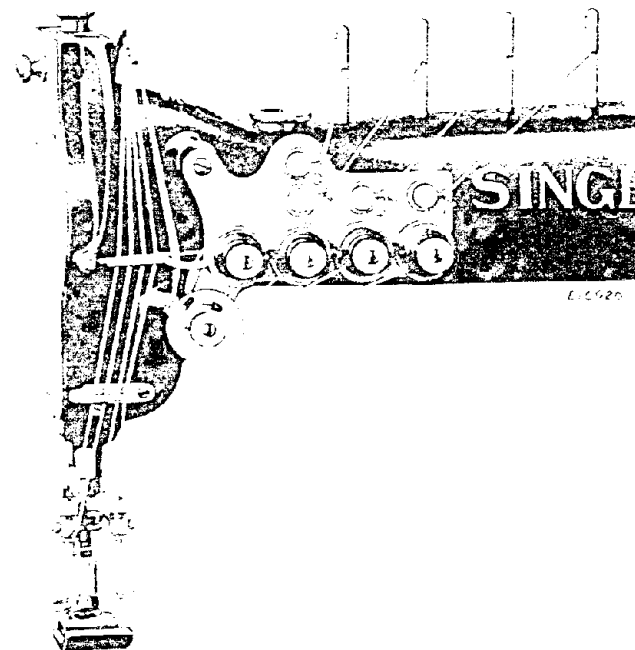
Fig. 14. Threading the Needles in Machines 131w104, 131w112 and 131w113
