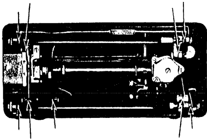
Fig. 6. Oiling Points in Base of Machine
