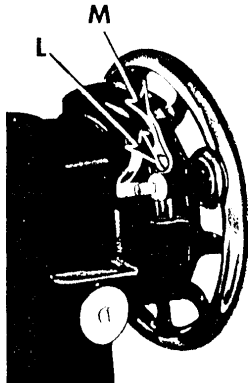
Fig. 16. Adjusting Bobbin Winder
