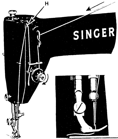
Fig. 10. Upper Threading Fig. 11. Threading Needle
