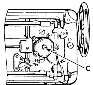
Fig. 5. Lower Gear Lubrication
