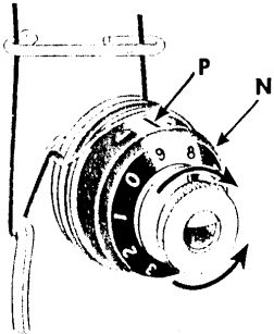
Fig. 25. Regulating Needle Thread Tension
