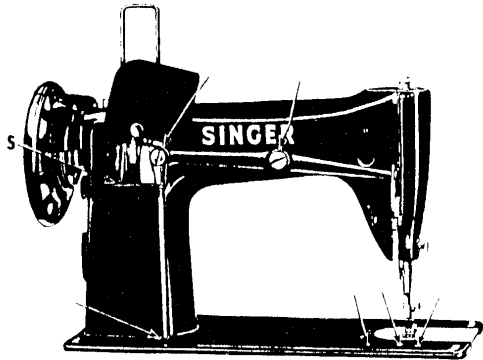
Fig. 3. Rear View—Oiling Points
