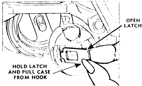
Fig. 12. Removing Bobbin Case from Sewing Hook
