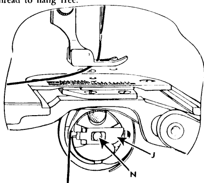
Fig. 20. Bobbin Case Threaded and Replaced
